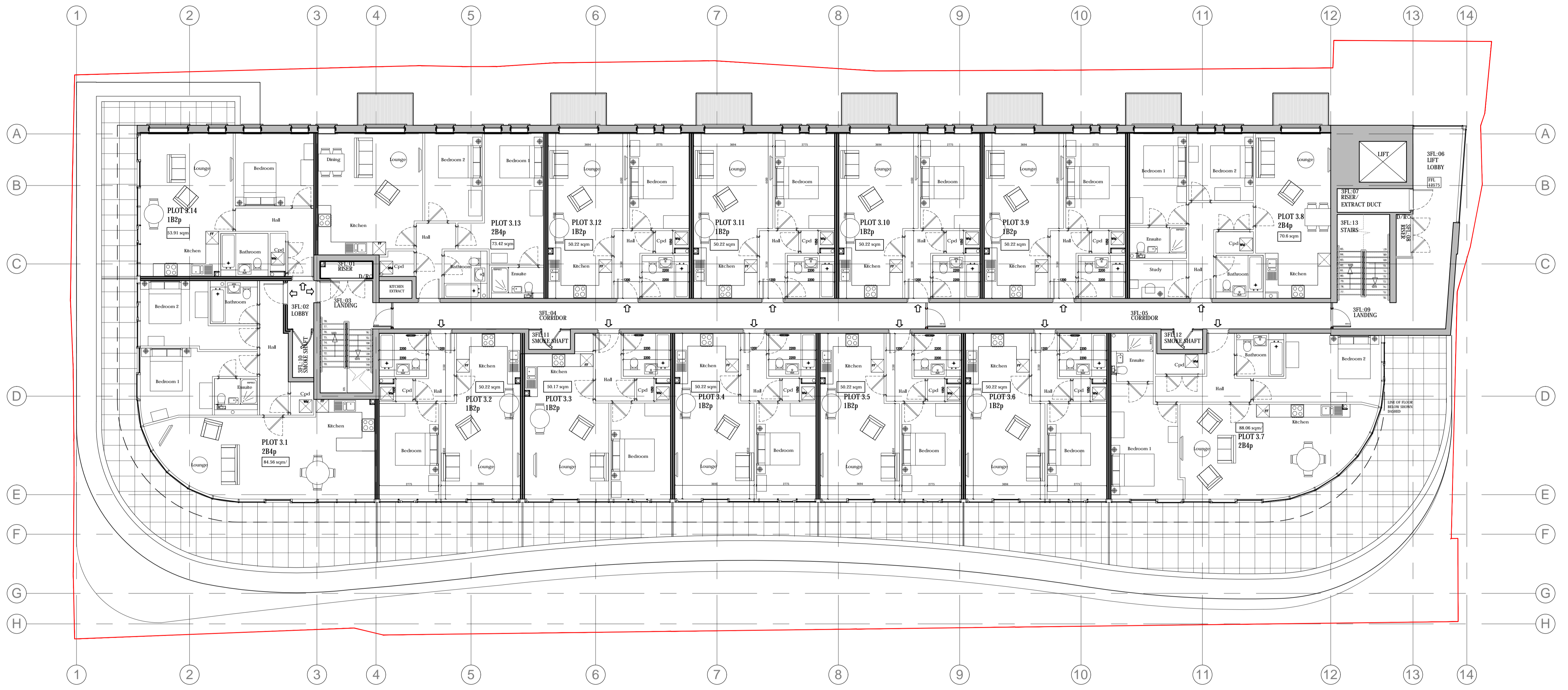
THIRD FLOOR Scale 1:100
